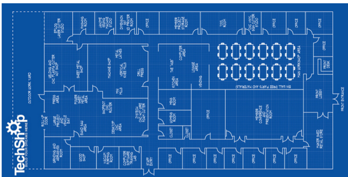
Figure 2 - Plan TechShop Menlow Park (URL : http://www.techshop.ws/Floor_Plan.html )
